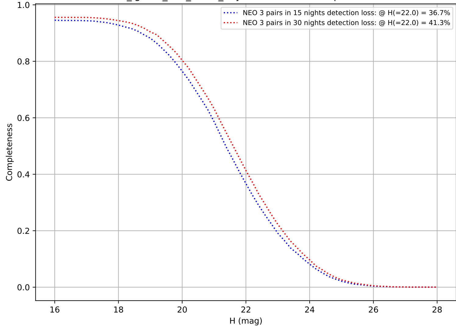
too_ignore_100_4v3.4_10yrs: DifferentialCompleteness
