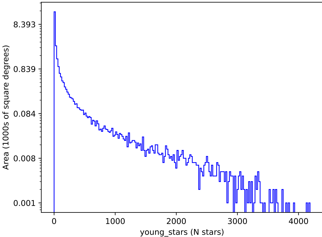
too_ignore_100_4v3.4_10yrs : young_stars
