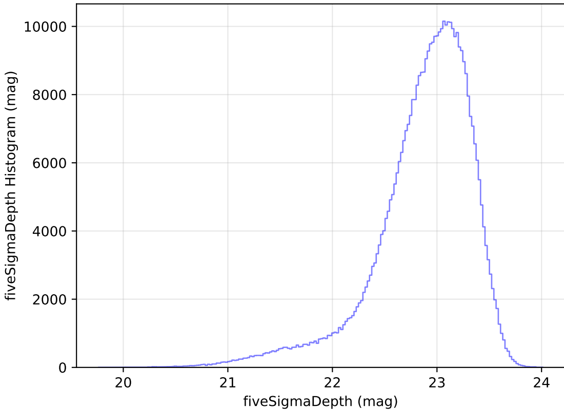
too_ignore_100_4v3.4_10yrs z: fiveSigmaDepth Histogram
