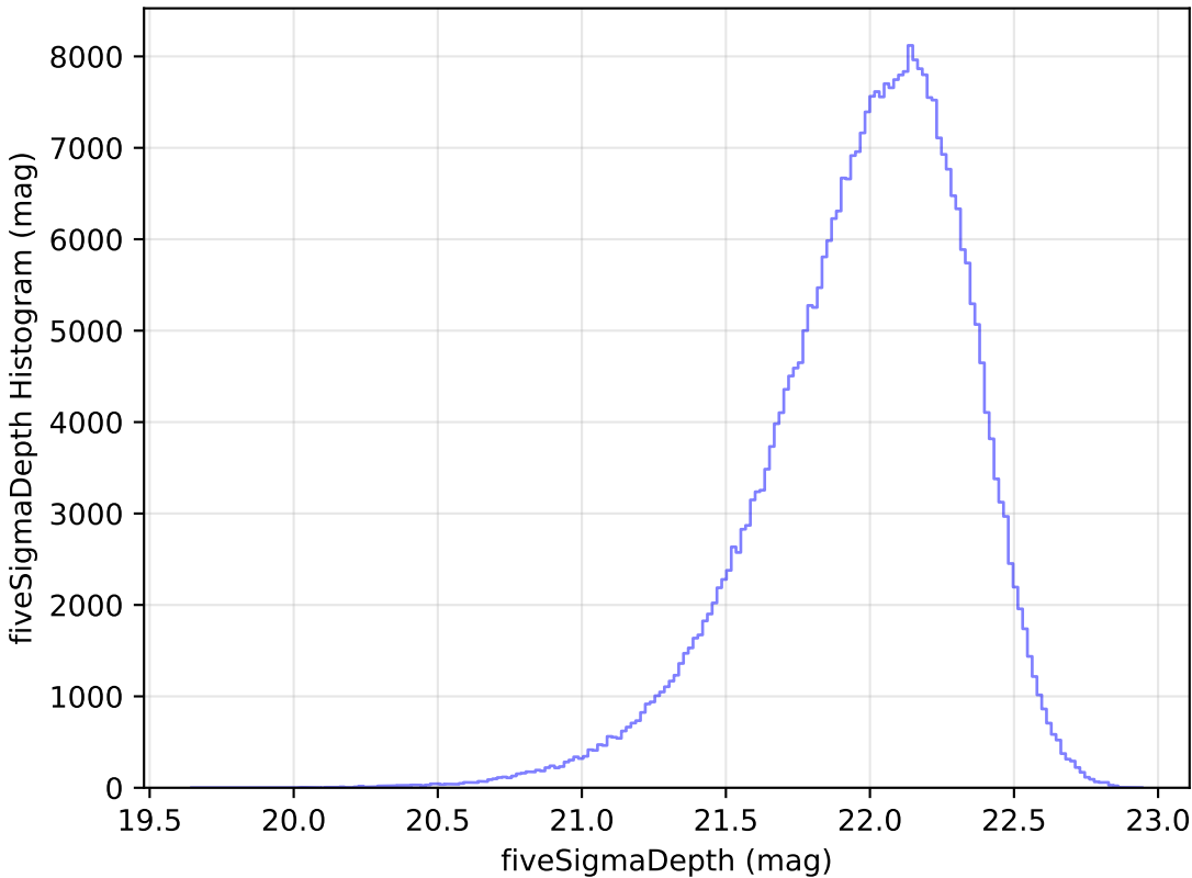
too_ignore_100_4v3.4_10yrs y: fiveSigmaDepth Histogram
