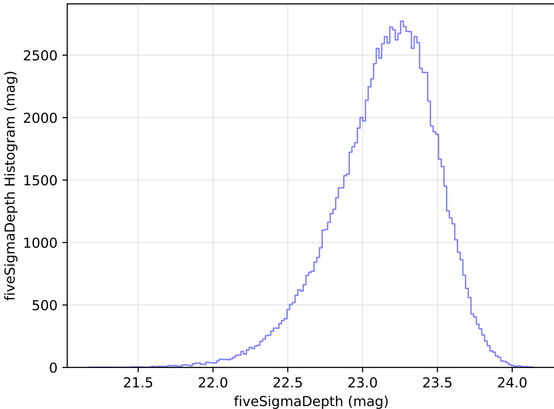
too_ignore_100_4v3.4_10yrs u: fiveSigmaDepth Histogram
