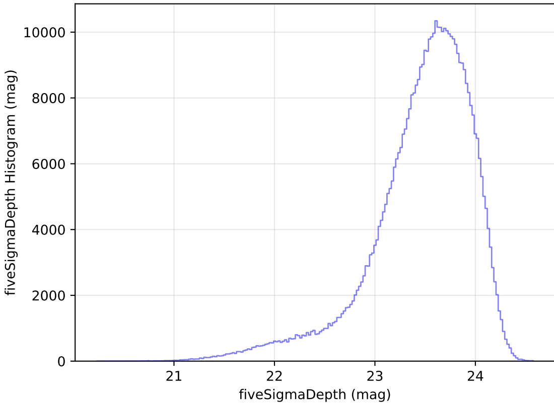
too_ignore_100_4v3.4_10yrs i: fiveSigmaDepth Histogram
