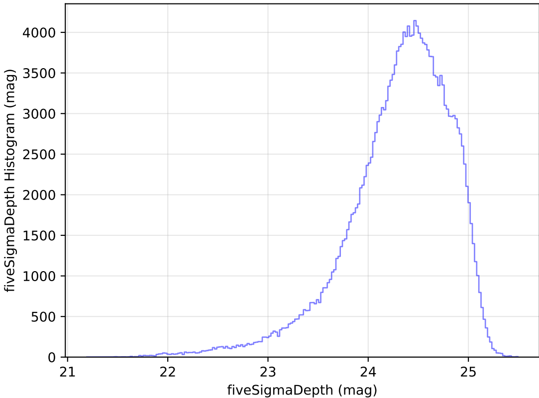
too_ignore_100_4v3.4_10yrs g: fiveSigmaDepth Histogram
