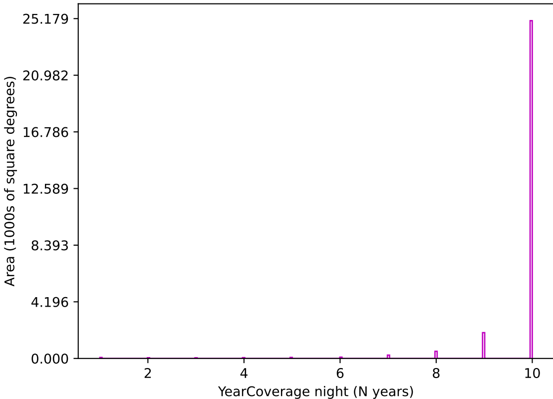
too_ignore_100_4v3.4_10yrs z band: YearCoverage night
