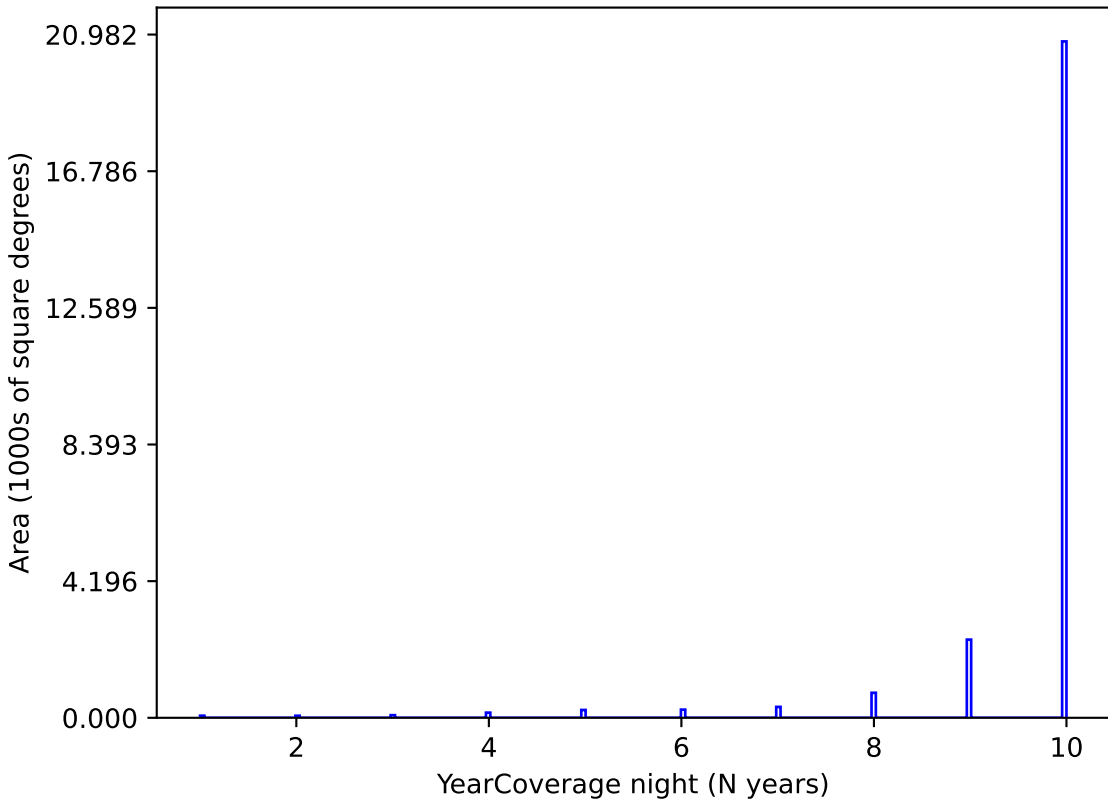
too_ignore_100_4v3.4_10yrs y band: YearCoverage night
