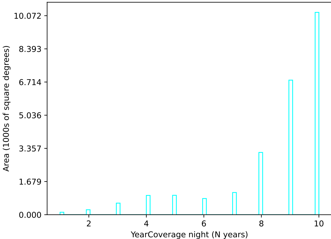
too_ignore_100_4v3.4_10yrs u band: YearCoverage night
