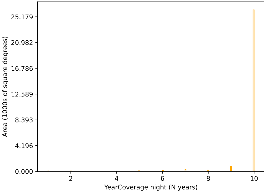
too_ignore_100_4v3.4_10yrs r band: YearCoverage night
