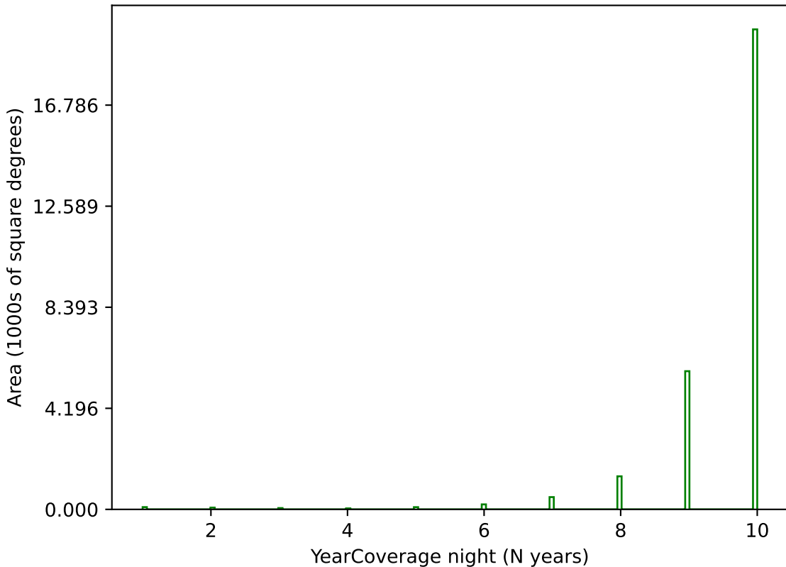
too_ignore_100_4v3.4_10yrs g band: YearCoverage night
