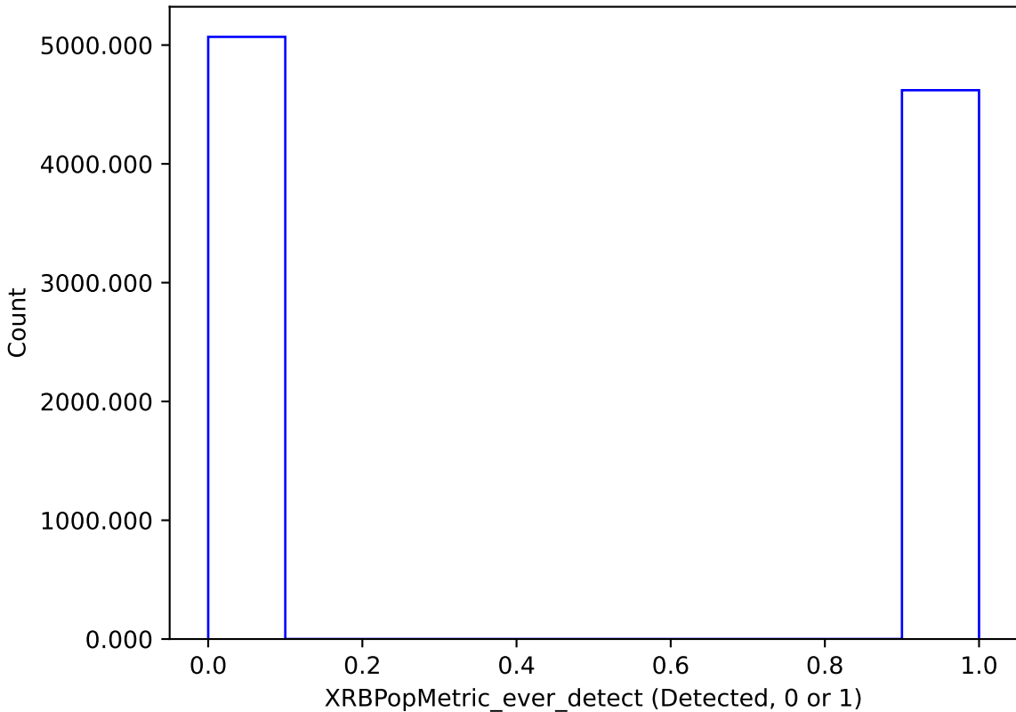
too_ignore_100_4v3.4_10yrs : XRBPoMetric_ever_detect
