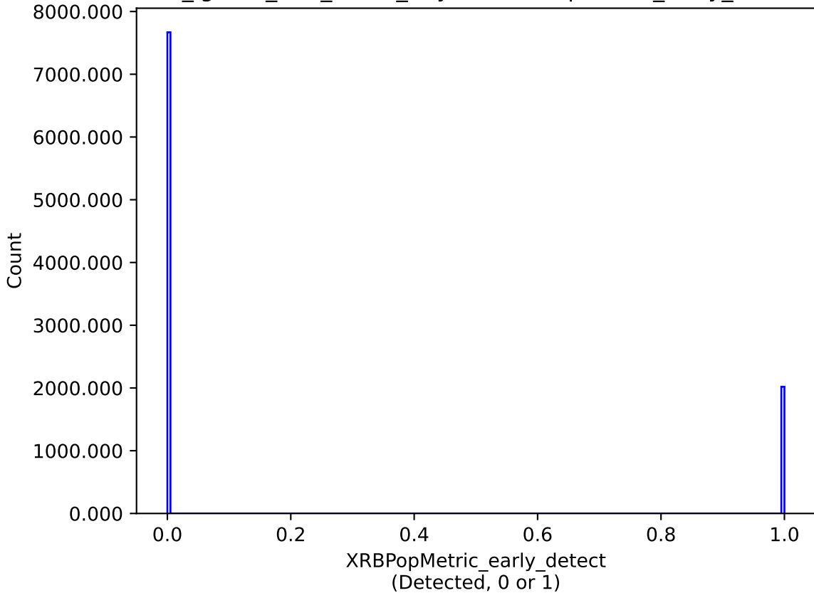
too_ignore_100_4v3.4_10yrs : XRBPoMetric_early_detect
