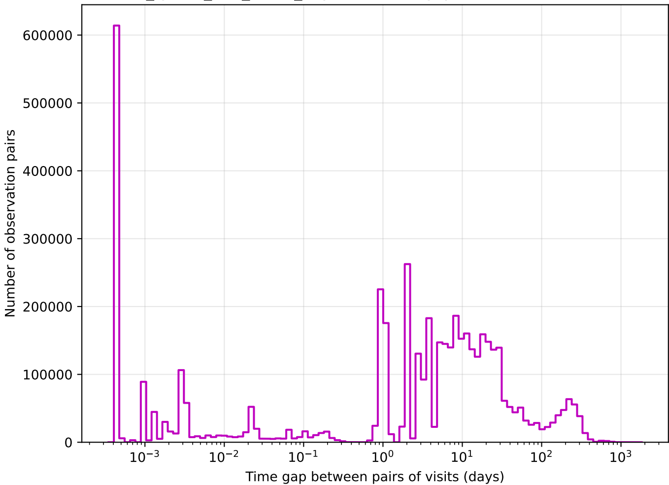
too_ignore_100_4v3.4_10yrs z band: Tgaps observationStartMJD
