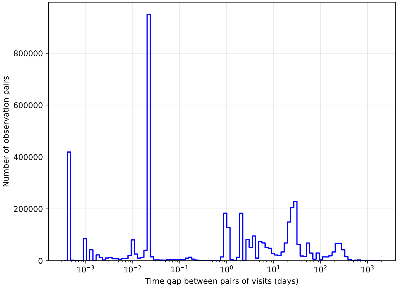
too_ignore_100_4v3.4_10yrs y band: Tgaps observationStartMJD
