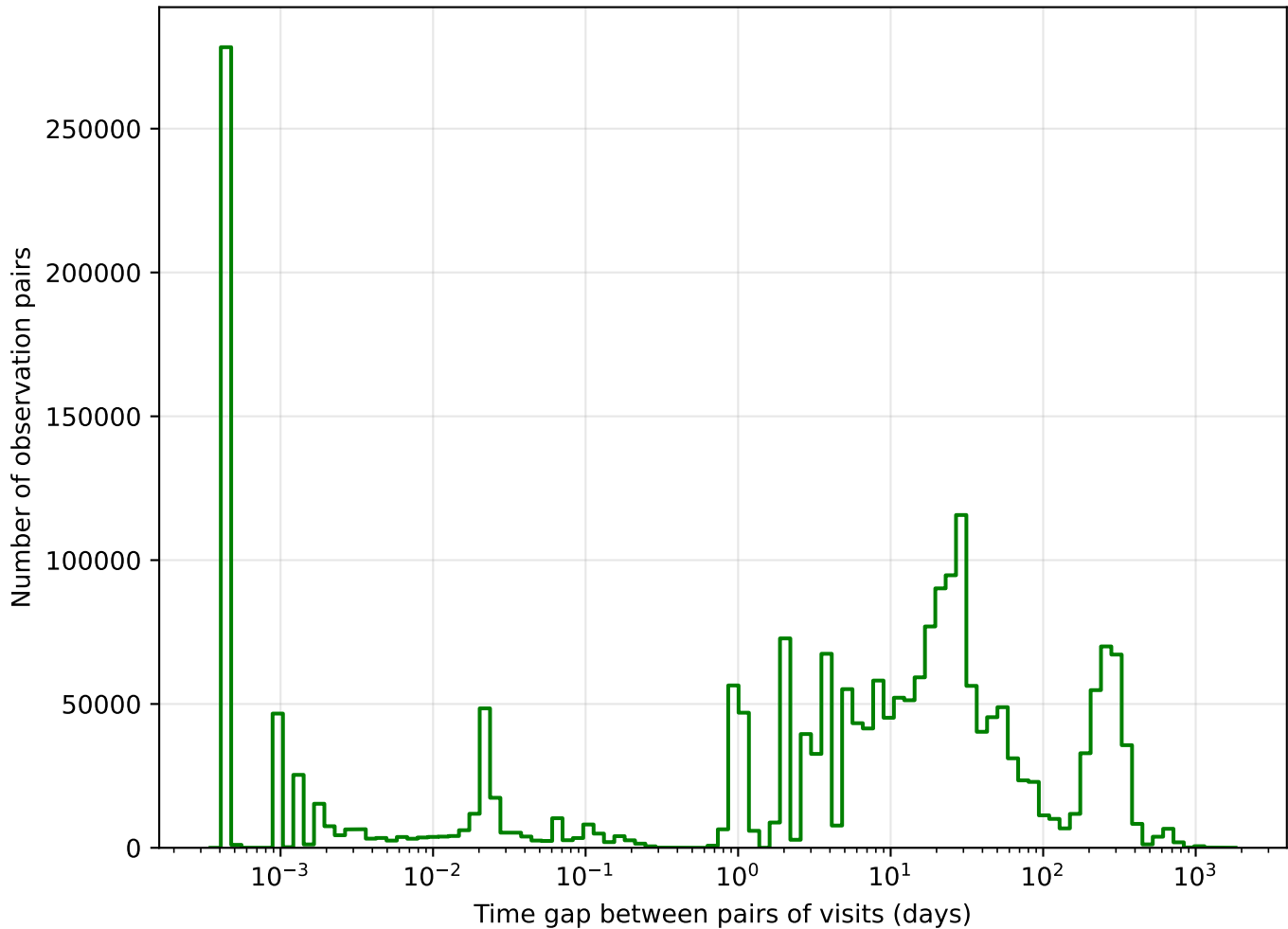
too_ignore_100_4v3.4_10yrs g band: Tgaps observationStartMJD
