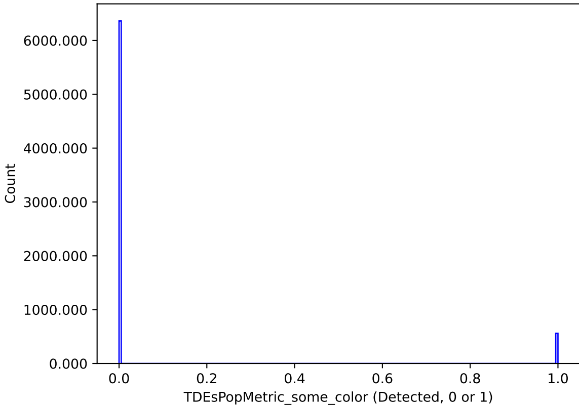
too_ignore_100_4v3.4_10yrs : TDEsPopMetric_some_color
