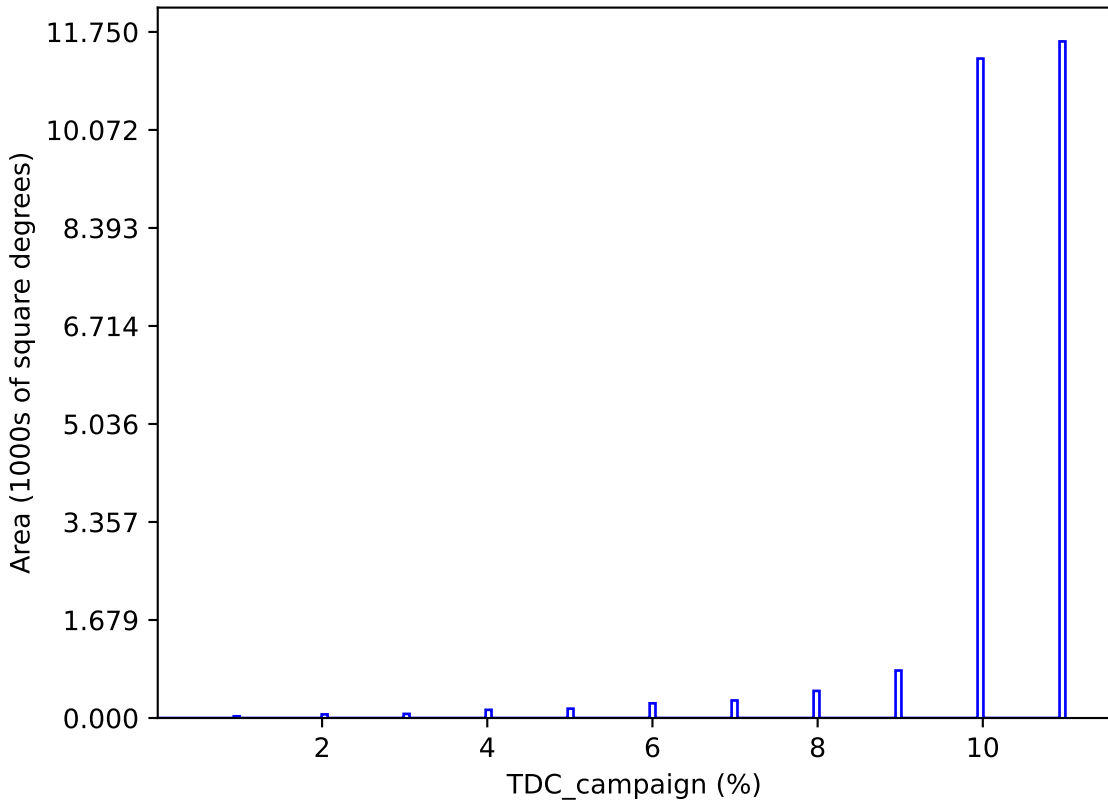
too_ignore_100_4v3.4_10yrs : TDC_campaign
