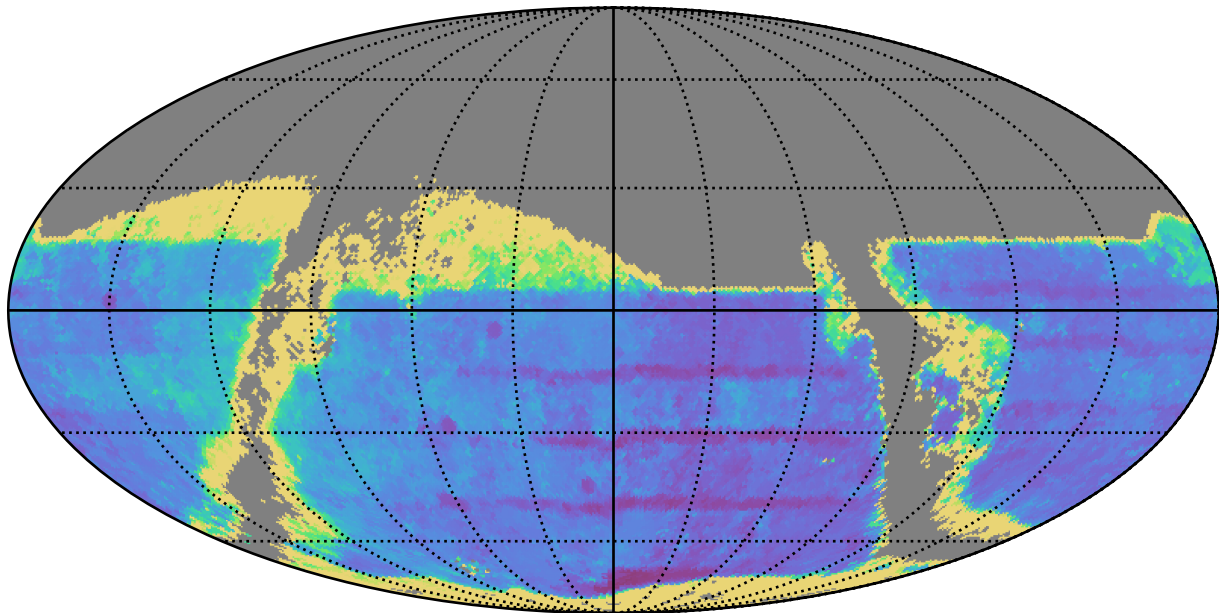
too_ignore_100_4v3.4_10yrs : TDC_accuracy
