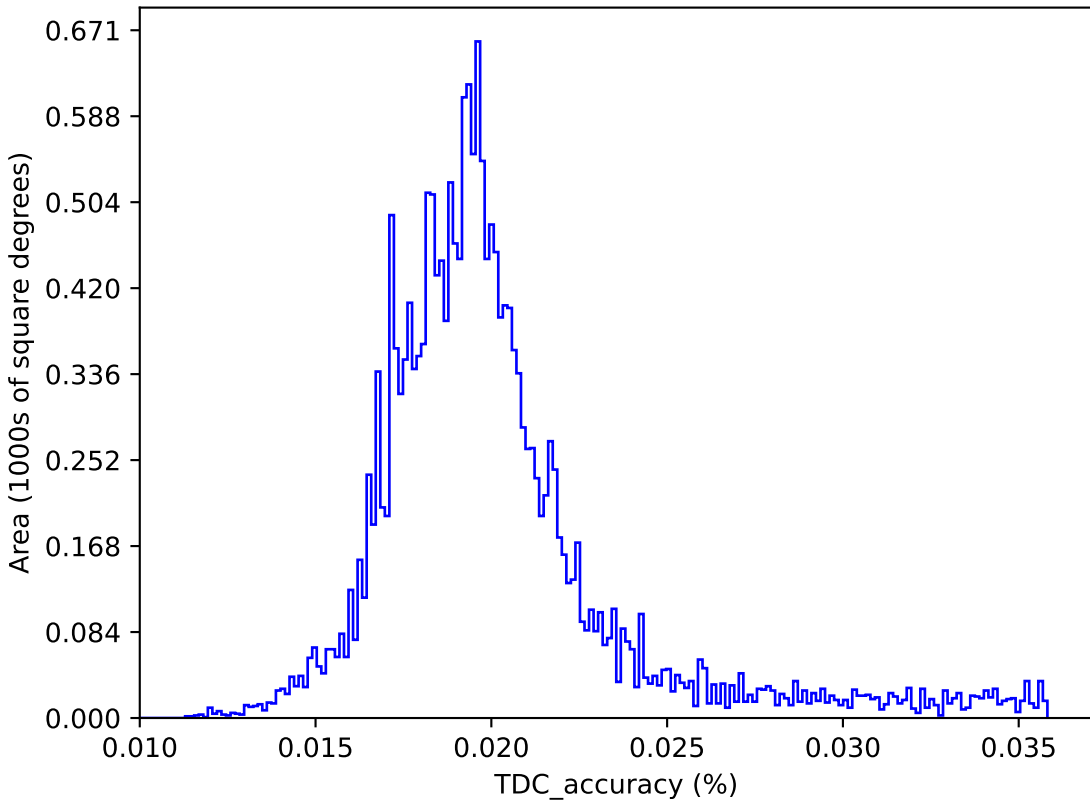
too_ignore_100_4v3.4_10yrs : TDC_accuracy
