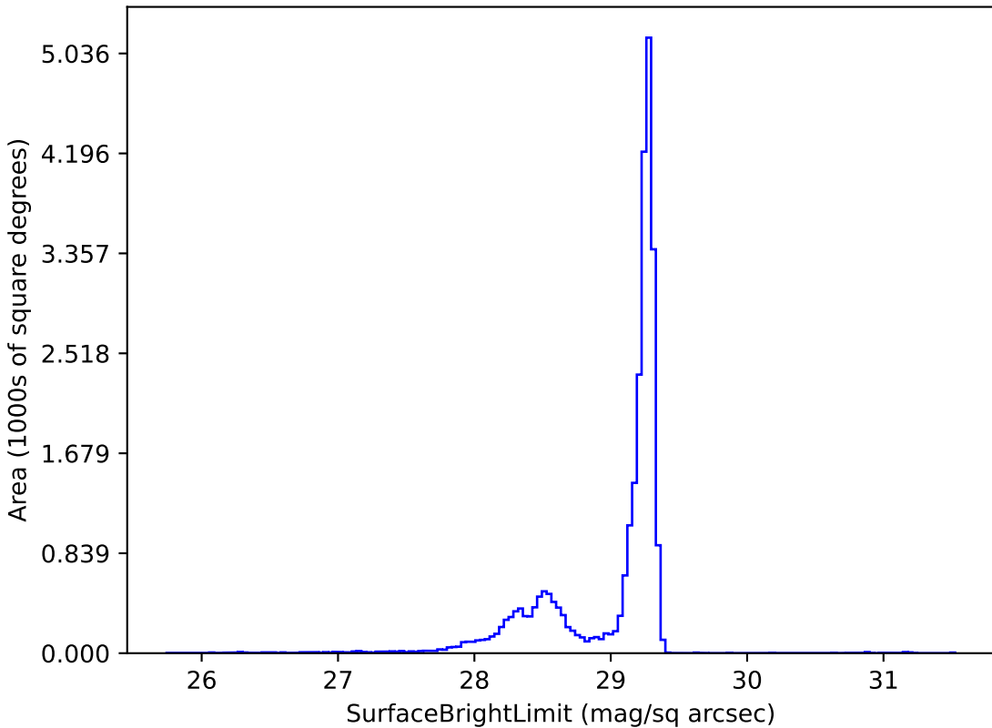
too_ignore_100_4v3.4_10yrs z: SurfaceBrightLimit
