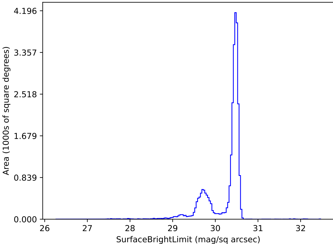
too_ignore_100_4v3.4_10yrs r: SurfaceBrightLimit
