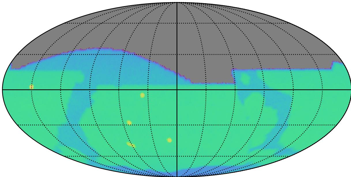
too_ignore_100_4v3.4_10yrs i: SurfaceBrightLimit
