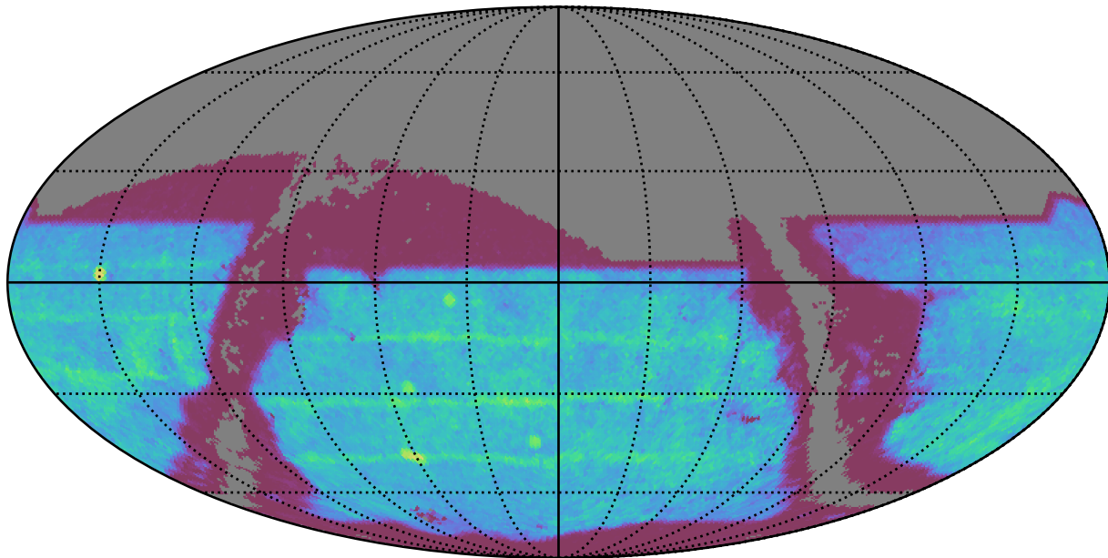
too_ignore_100_4v3.4_10yrs : SNSLMetric
