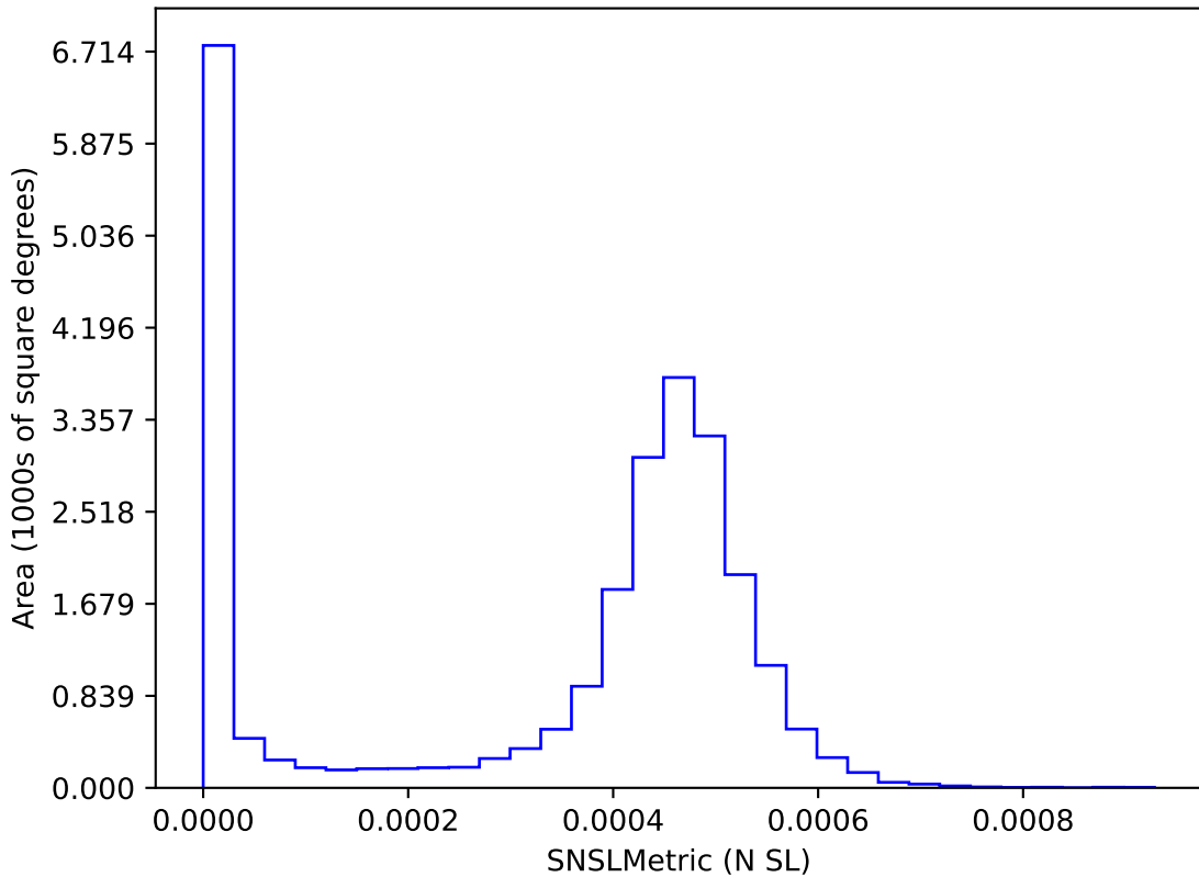
too_ignore_100_4v3.4_10yrs : SNSLMetric
