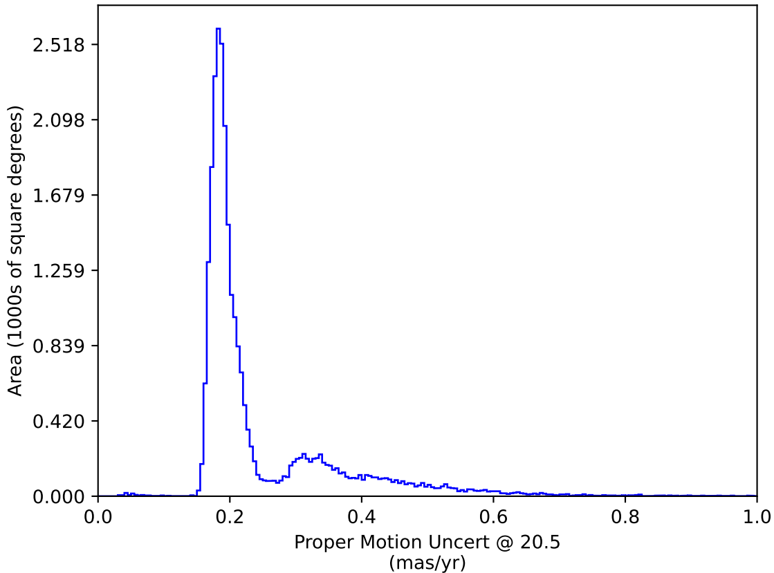
too_ignore_100_4v3.4_10yrs : Proper Motion Uncert @ 20.5
