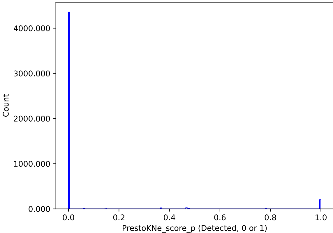
too_ignore_100_4v3.4_10yrs : PrestoKNe_score_p
