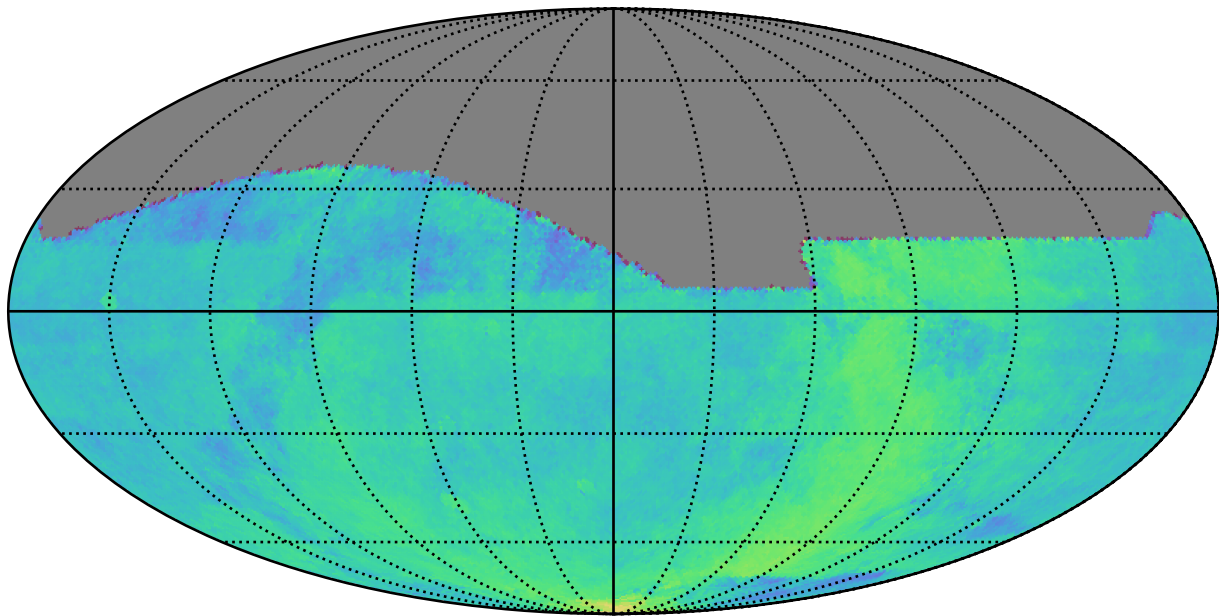
too_ignore_100_4v3.4_10yrs : Parallax Coverage @ 24.0
