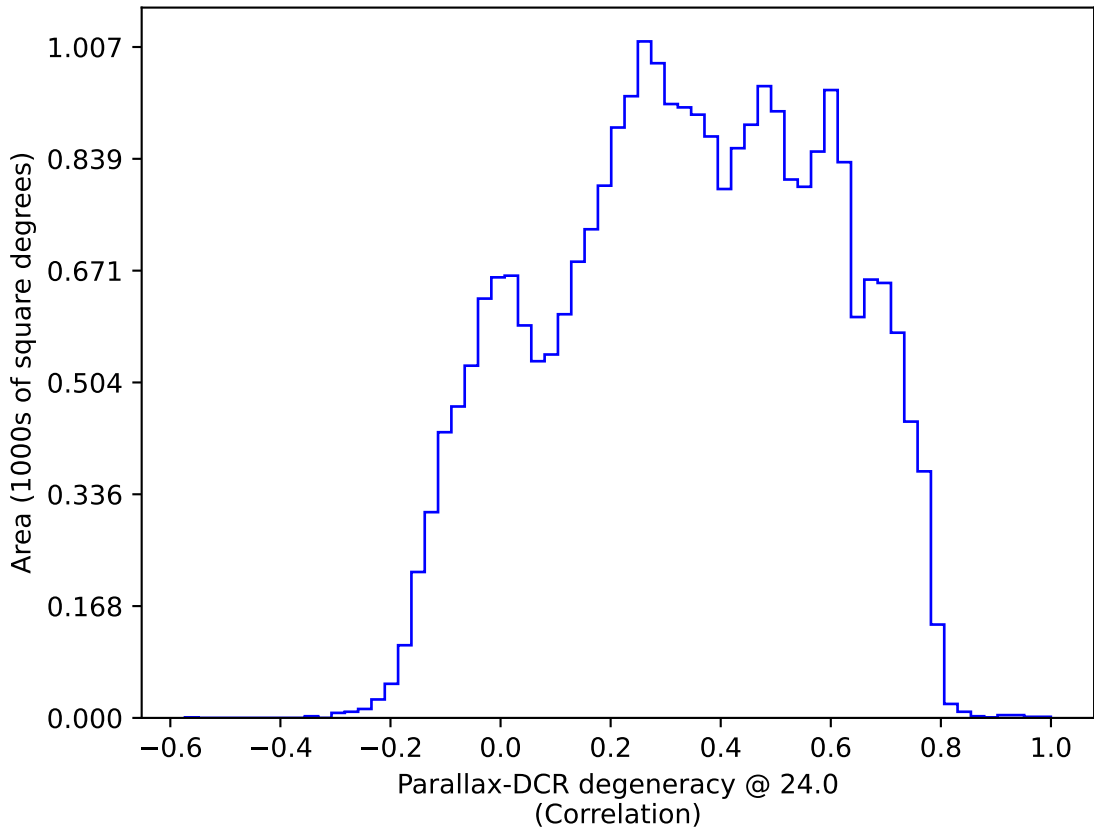
too_ignore_100_4v3.4_10yrs : Parallax-DCR degeneracy @ 24.0
