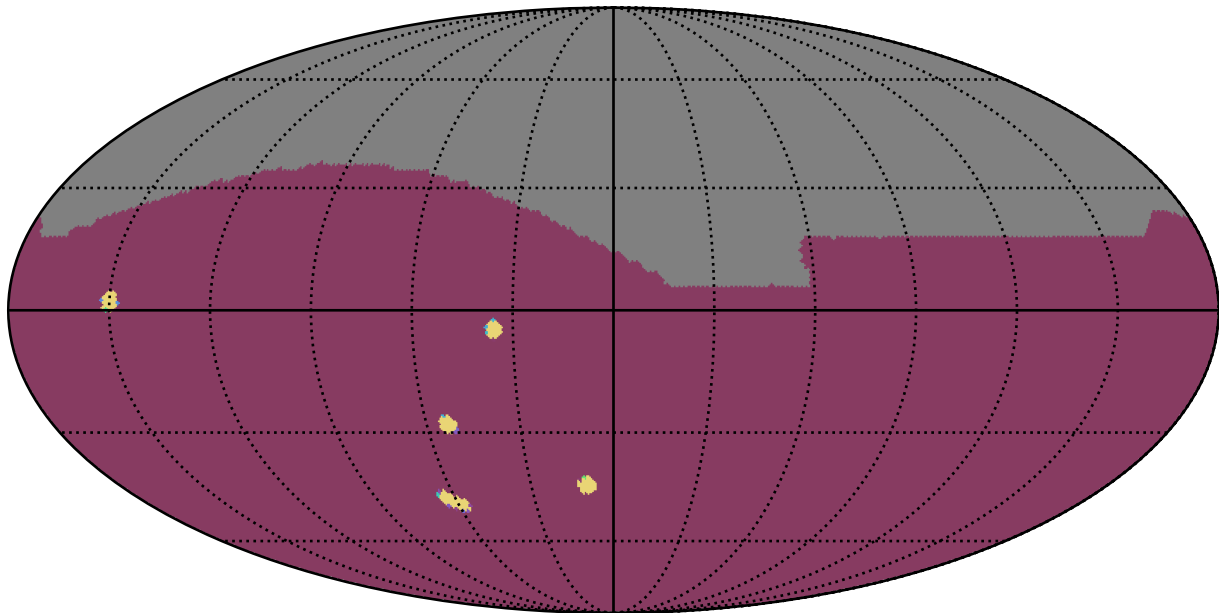
too_ignore_100_4v3.4_10yrs : NumberOfQuickRevisits
