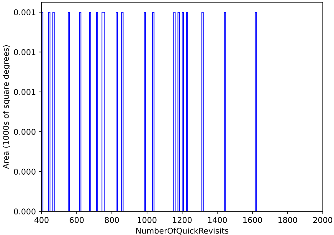
too_ignore_100_4v3.4_10yrs : NumberOfQuickRevisits
