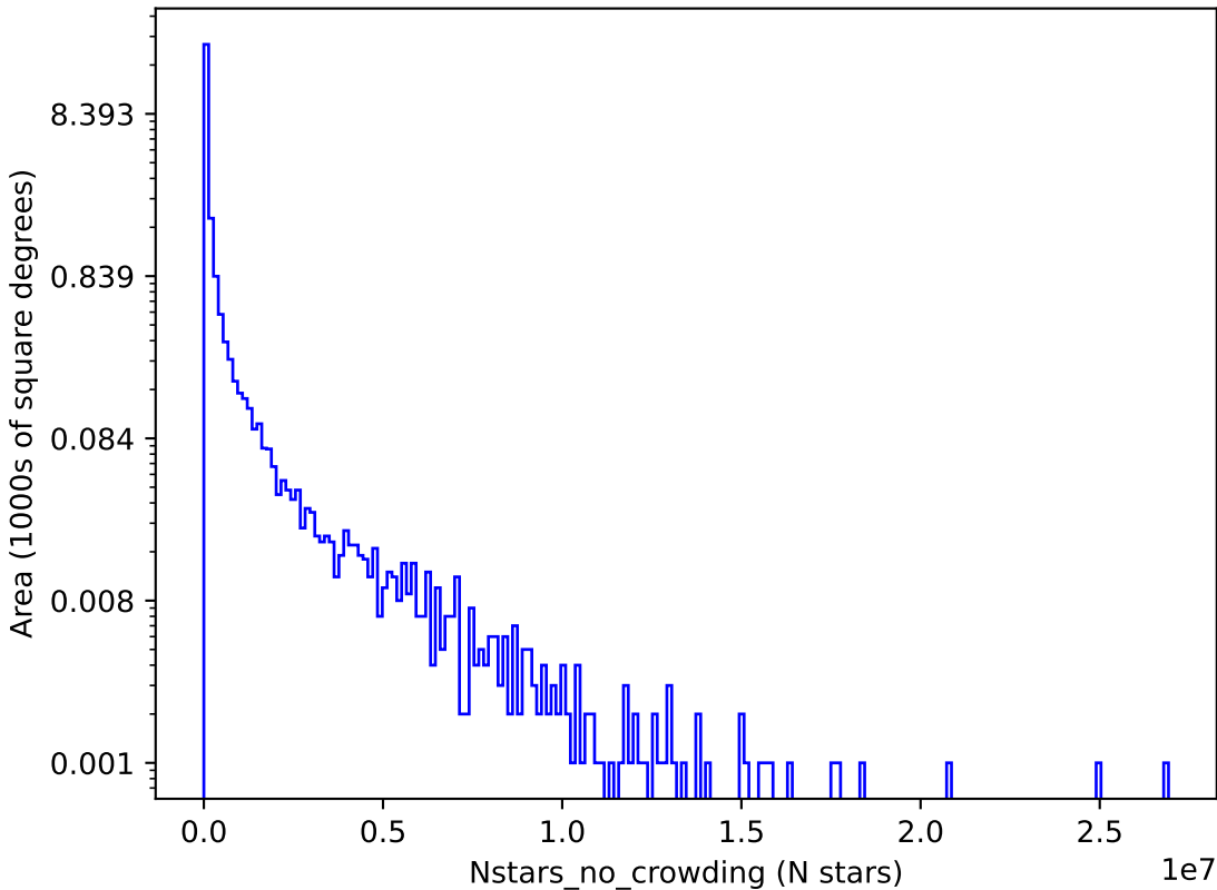
too_ignore_100_4v3.4_10yrs z: Nstars_no_crowding
