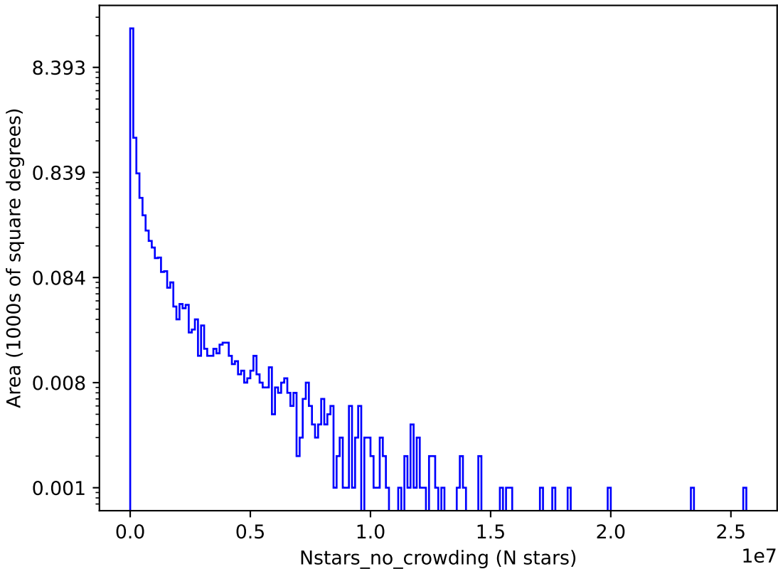
too_ignore_100_4v3.4_10yrs y: Nstars_no_crowding
