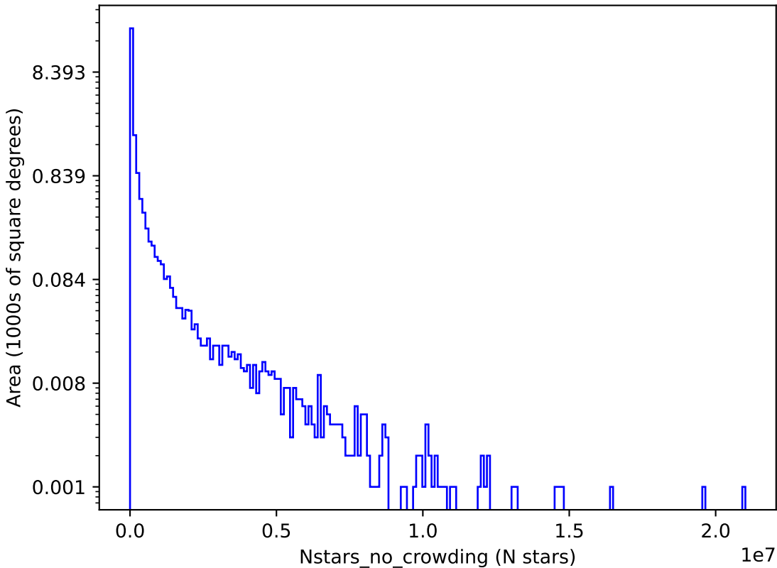
too_ignore_100_4v3.4_10yrs r: Nstars_no_crowding
