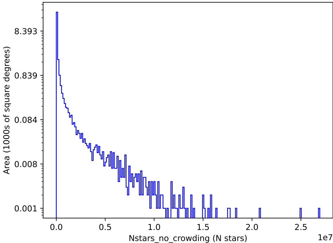
too_ignore_100_4v3.4_10yrs i: Nstars_no_crowding
