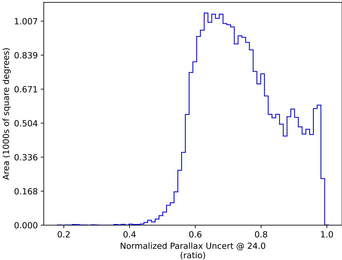
too_ignore_100_4v3.4_10yrs : Normalized Parallax Uncert @ 24.0
