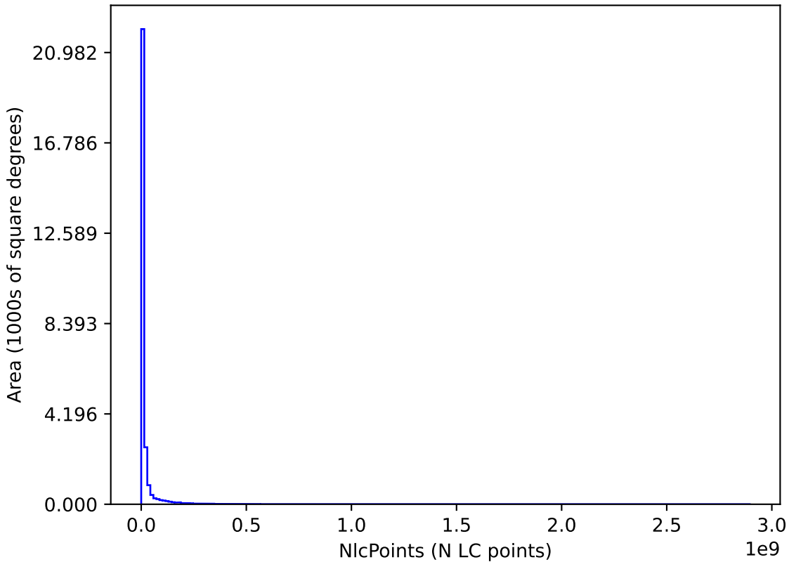
too_ignore_100_4v3.4_10yrs : NlcPoints
