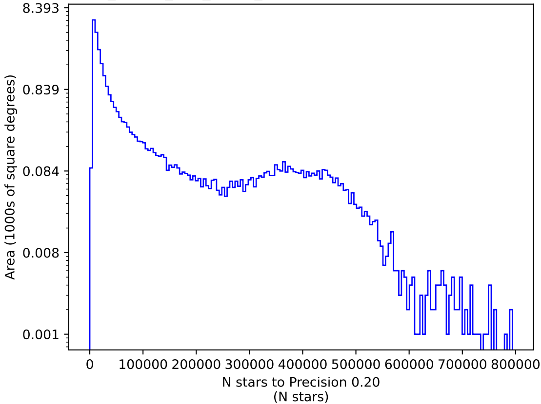
too_ignore_100_4v3.4_10yrs z: N stars to Precision 0.20
