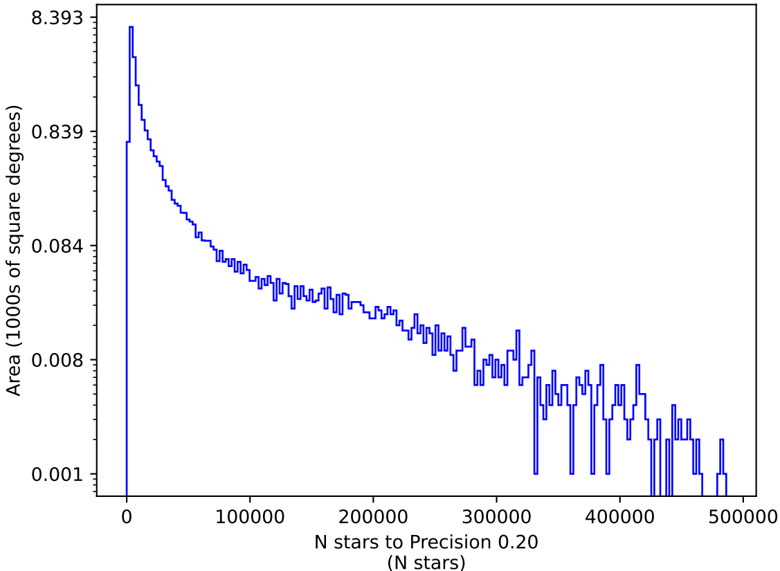
too_ignore_100_4v3.4_10yrs u: N stars to Precision 0.20
