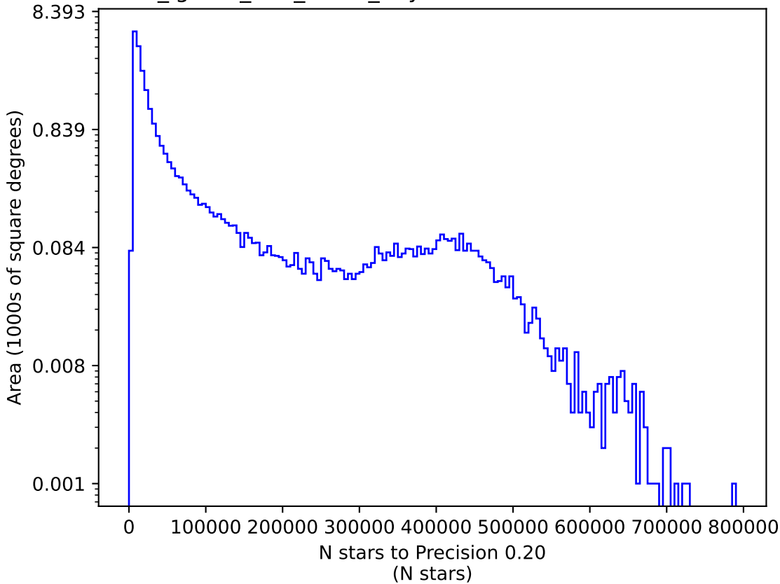
too_ignore_100_4v3.4_10yrs i: N stars to Precision 0.20
