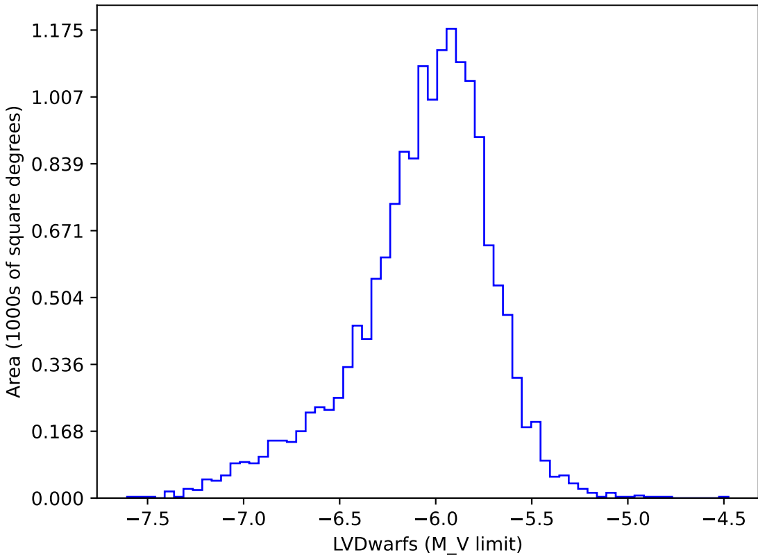
too_ignore_100_4v3.4_10yrs gi: LVDwarfs
