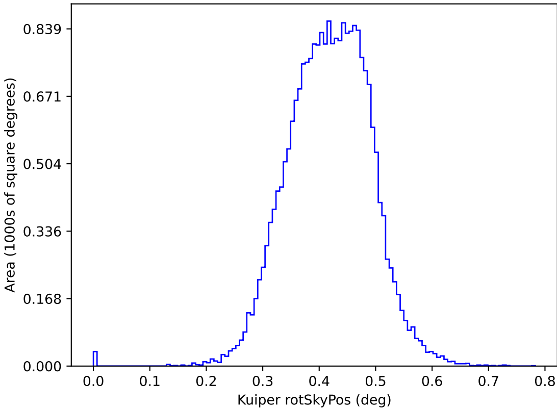
too_ignore_100_4v3.4_10yrs y: Kuiper rotSkyPos
