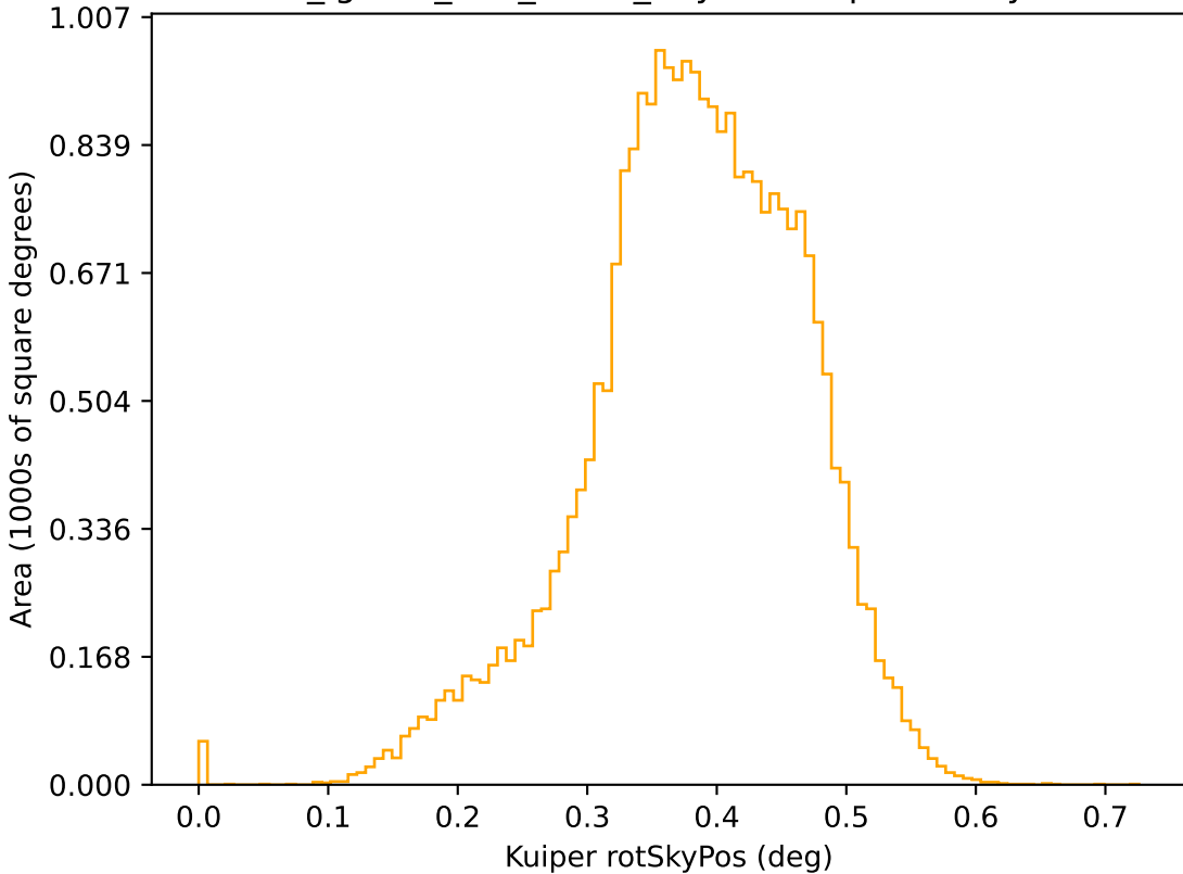
too_ignore_100_4v3.4_10yrs r: Kuiper rotSkyPos
