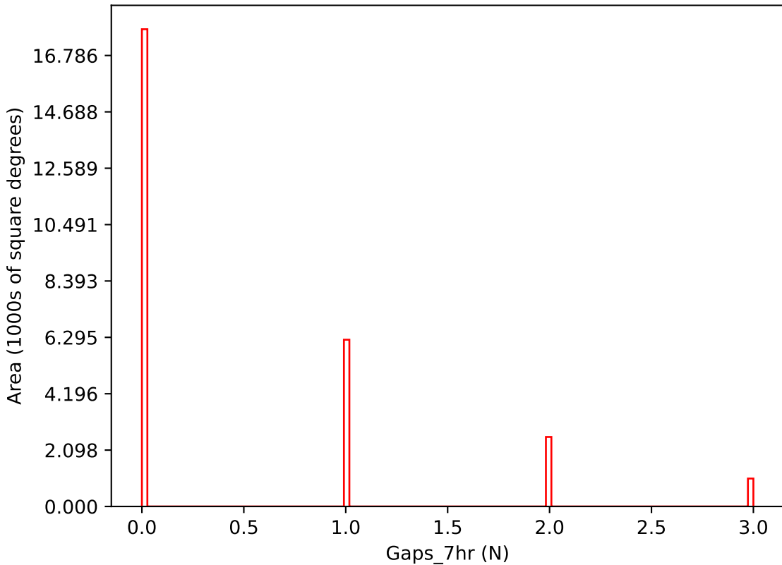
too_ignore_100_4v3.4_10yrs i band: Gaps_7hr
