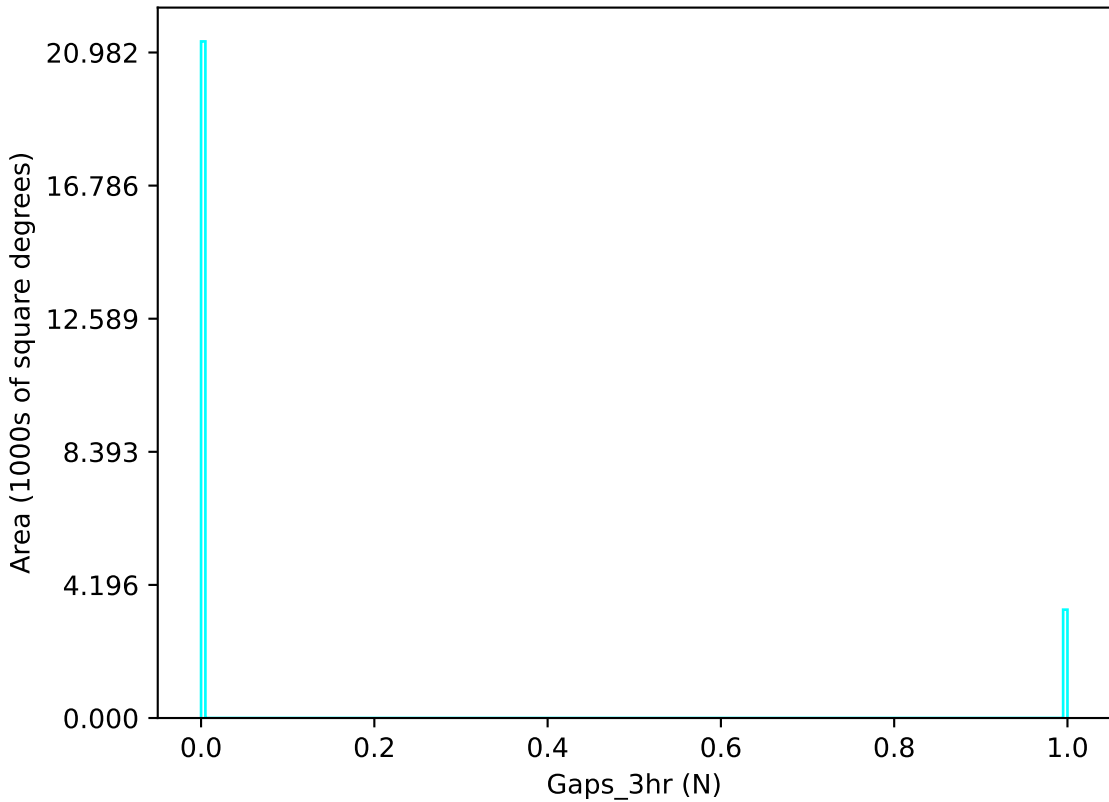
too_ignore_100_4v3.4_10yrs u band: Gaps_3hr
