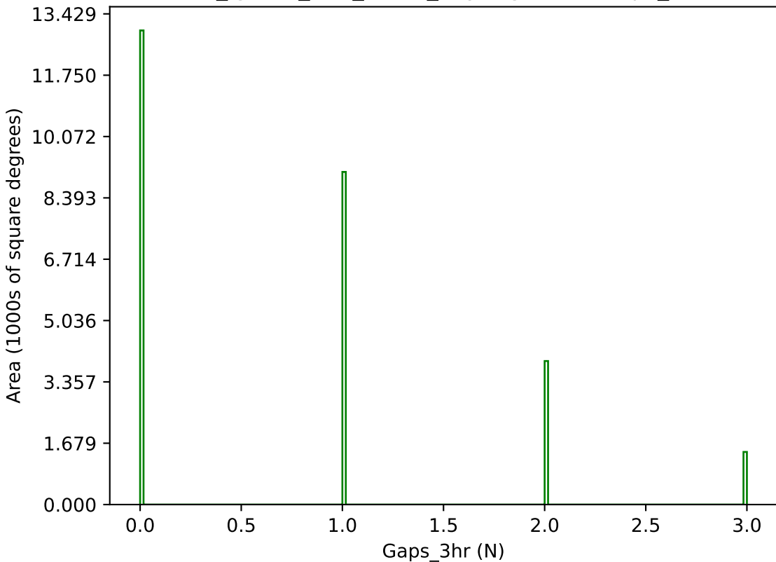
too_ignore_100_4v3.4_10yrs g band: Gaps_3hr
