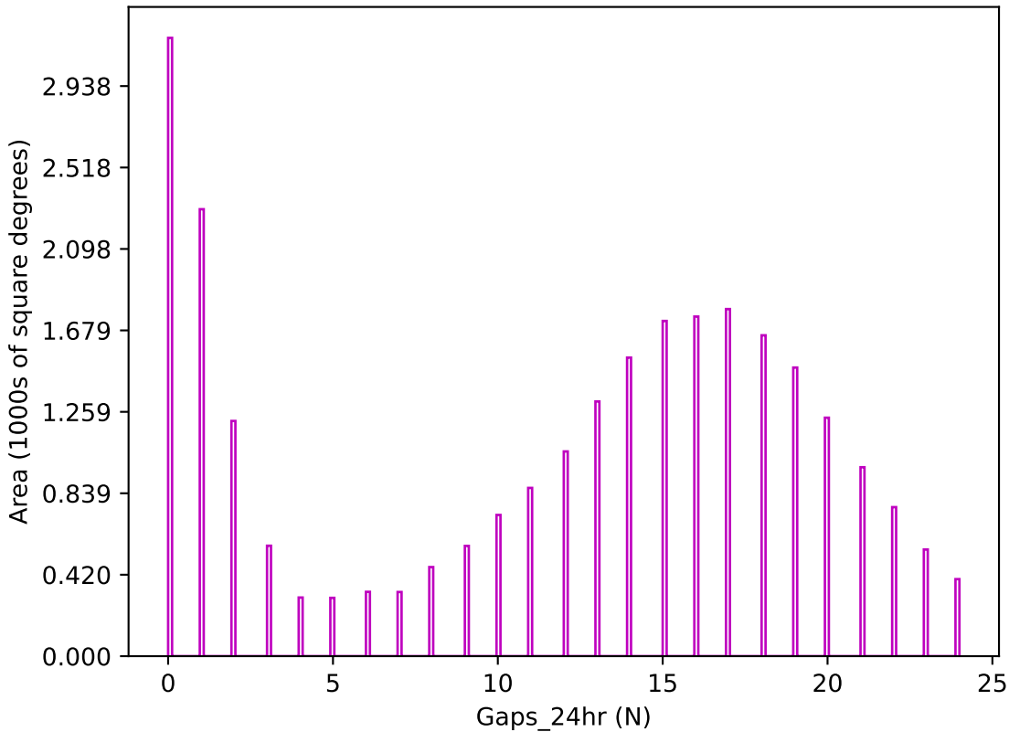
too_ignore_100_4v3.4_10yrs z band: Gaps_24hr
