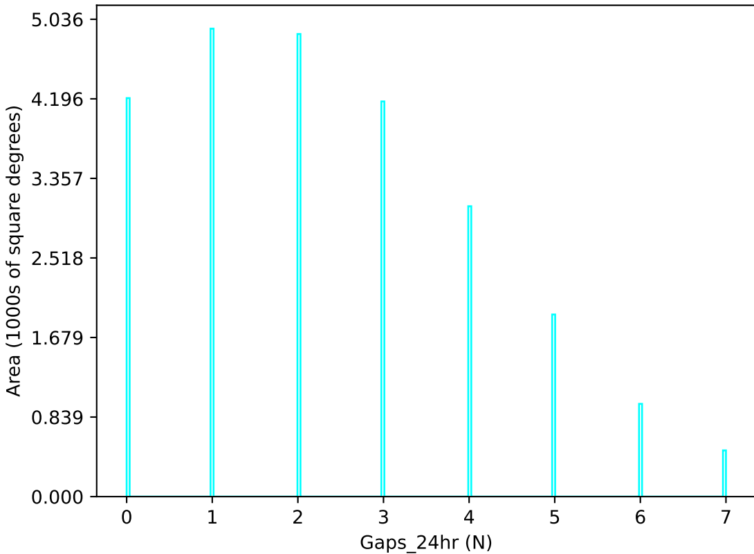
too_ignore_100_4v3.4_10yrs u band: Gaps_24hr
