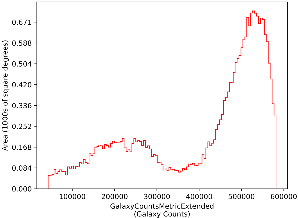
too_ignore_100_4v3.4_10yrs i: GalaxyCountsMetricExtended
